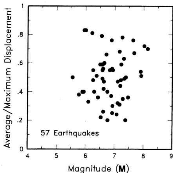
Figure 5. Ratio of average surface to maximum surface displacement versus magnitude.
