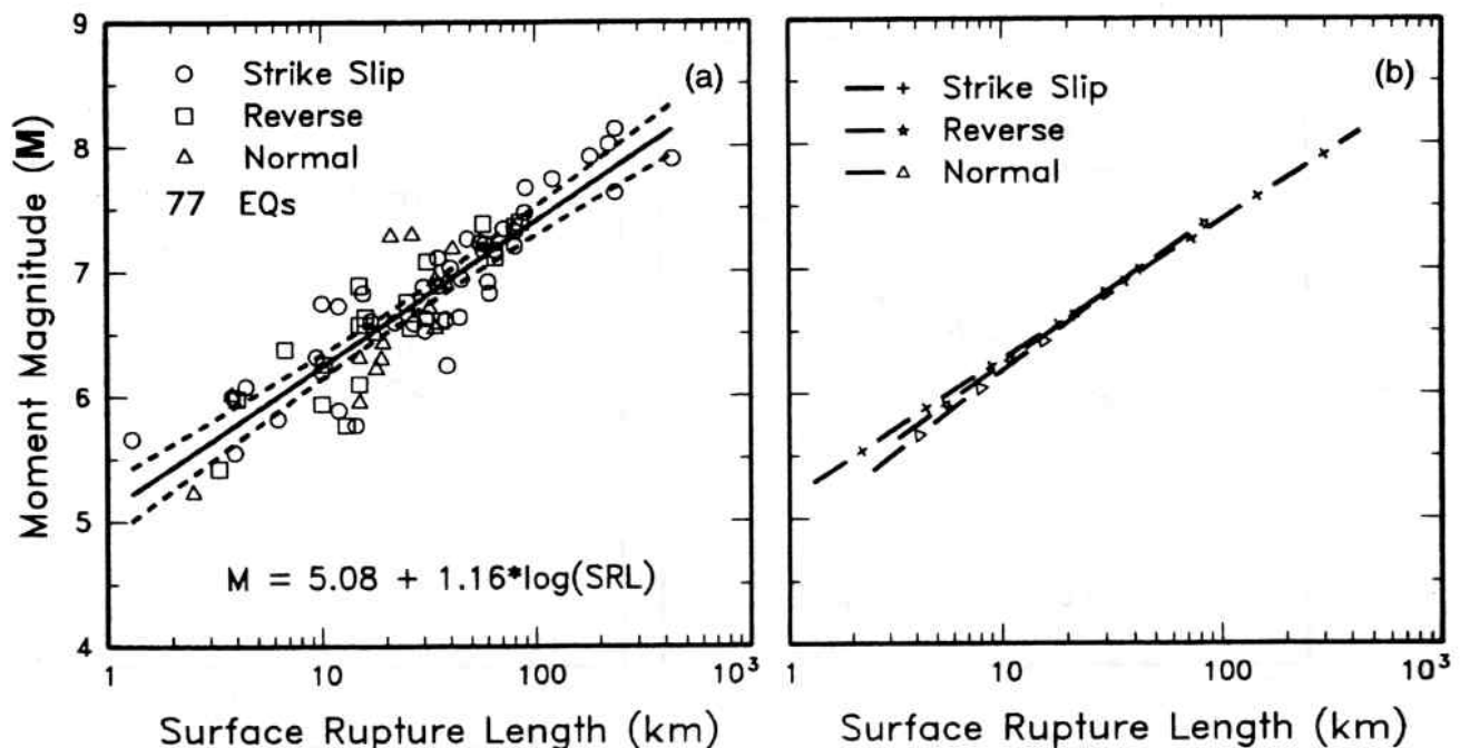
Figure 9. (a) Regression of surface rupture length on magnitude ( M ). Regression line shown for all-slip-type relationship. Short dashed line indicates 95% confidence interval. (b) Regression lines for strike-slip, reverse, and normal-slip relationships. See Table 2 for regression coefficients. Length of regression lines shows the range of data for each relationship.
