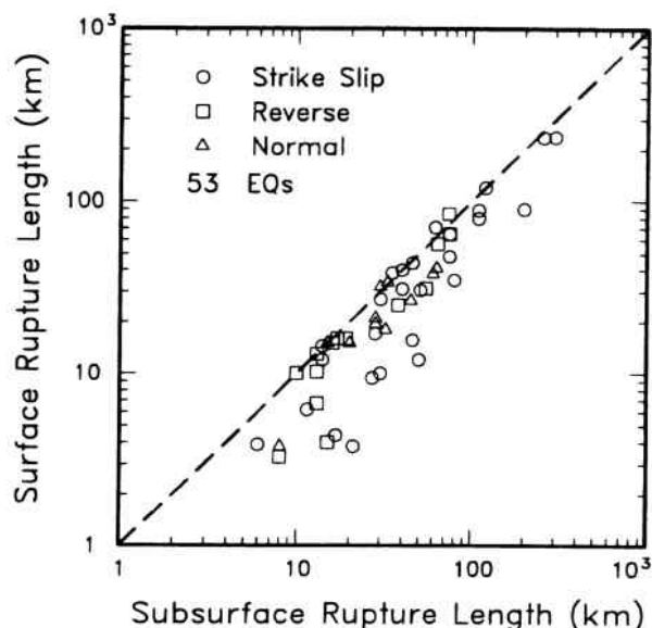
Figure 2. Surface rupture length versus subsurface rupture length estimated from the distribution of early aftershocks of historical continental earthquakes.
