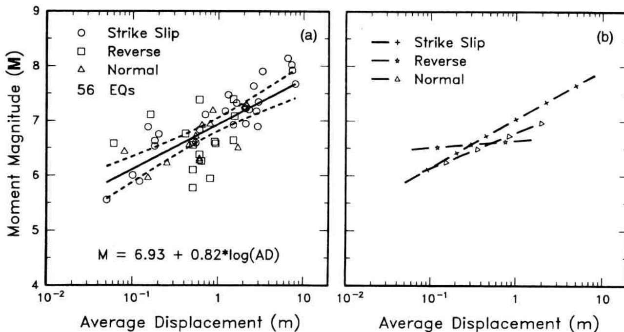
Figure 11. (a) Regression of average surface displacement on magnitude (M). Regression line shown for all-slip-type relationship. Short dashed line indicates 95% confidence interval. (b) Regression lines for strike-slip, reverse, and normal-slip relationships. See Table 2 for regression coefficients. Length of regression lines shows the range of data for each relationship.
