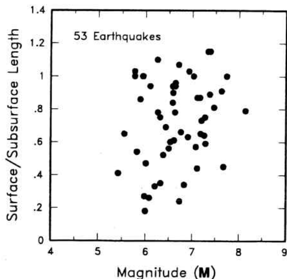
Figure 3. Ratio of surface to subsurface rupture length versus magnitude.
