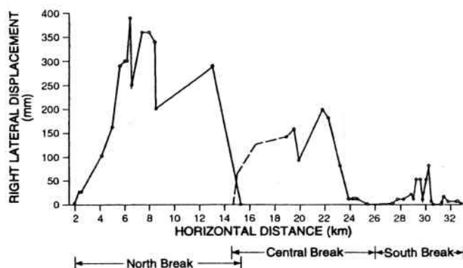
Figure 4. Distribution of right slip measured in April 1968 for the 9 April 1968 Borrego Mountain, California, earthquake. Dashed line indicates estimated displacement for April 1968 (modified from Clark, 1972).
