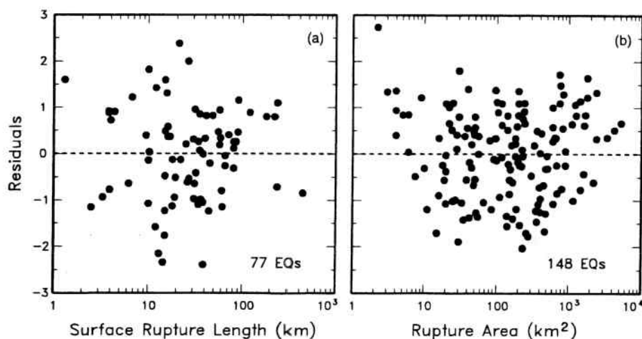
Figure 8. (a) Residuals for surface rupture length regression versus observed surface rupture length. (b) Residuals for rupture area regression versus observed rupture area.
